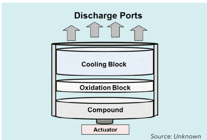
Typical Components of an Aerosol Generator
